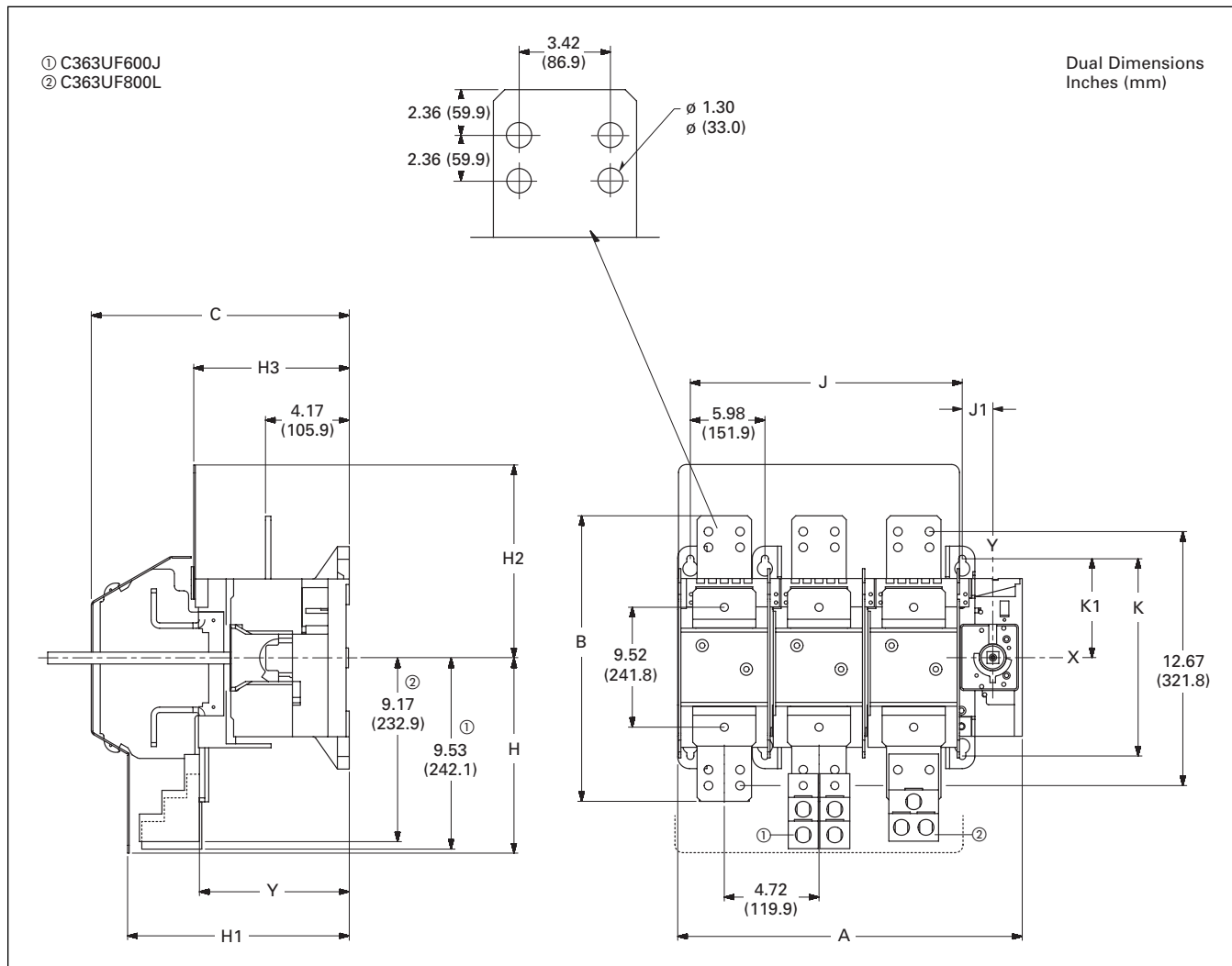
Figure 10. Fusible F-Frames
